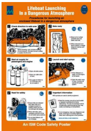
Lifeboat launching in a dangerous atmosphere
