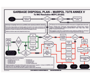
Garbage disposal plan
